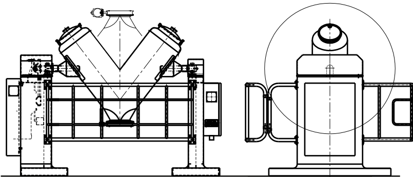
Vista Frontal Front view Vista Lateral Side view
